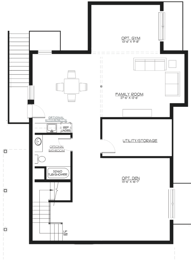
OPTIONAL LOWER LEVEL | 1,416 SF
