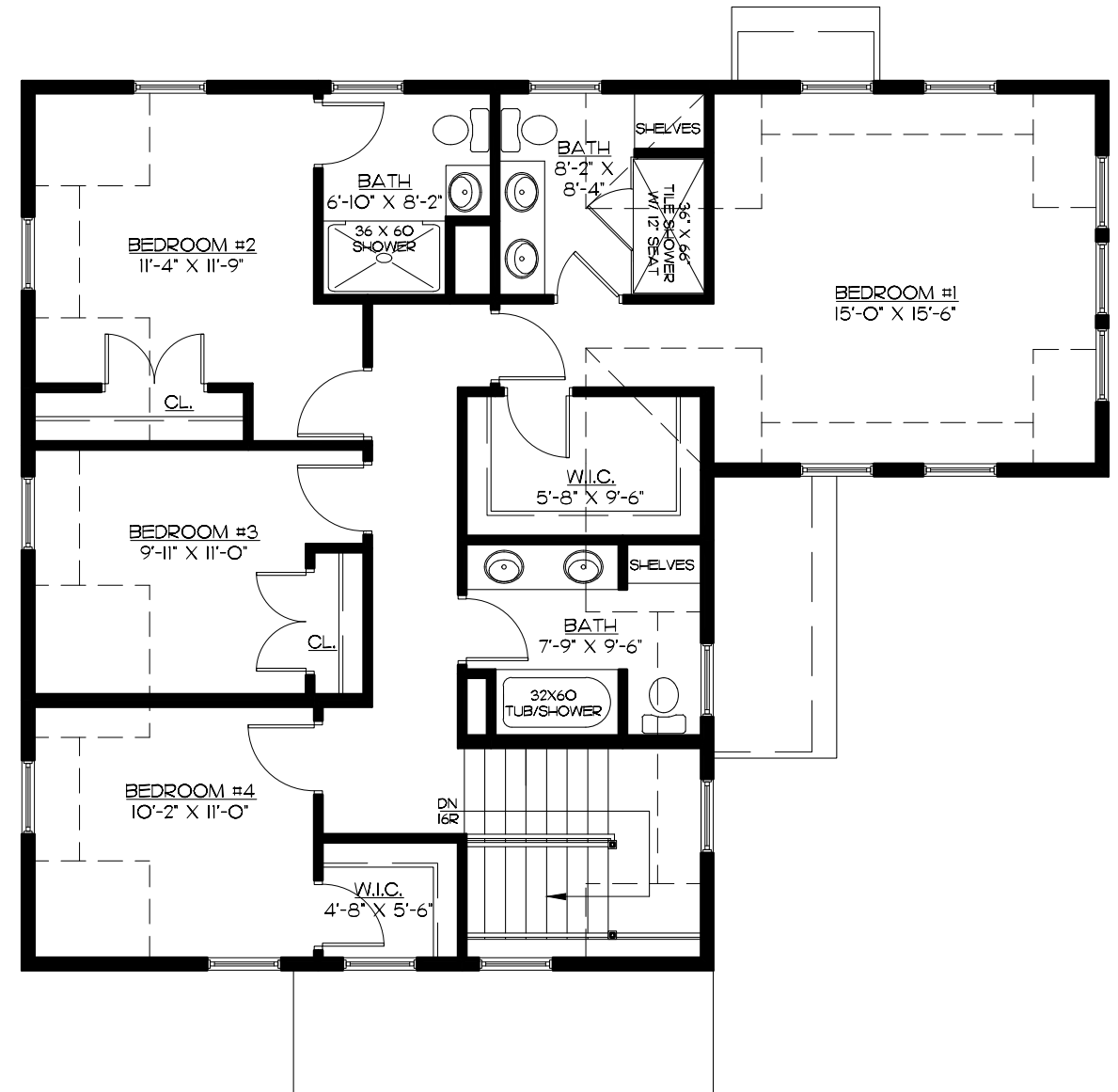
SECOND FLOOR | 1,220 SF
