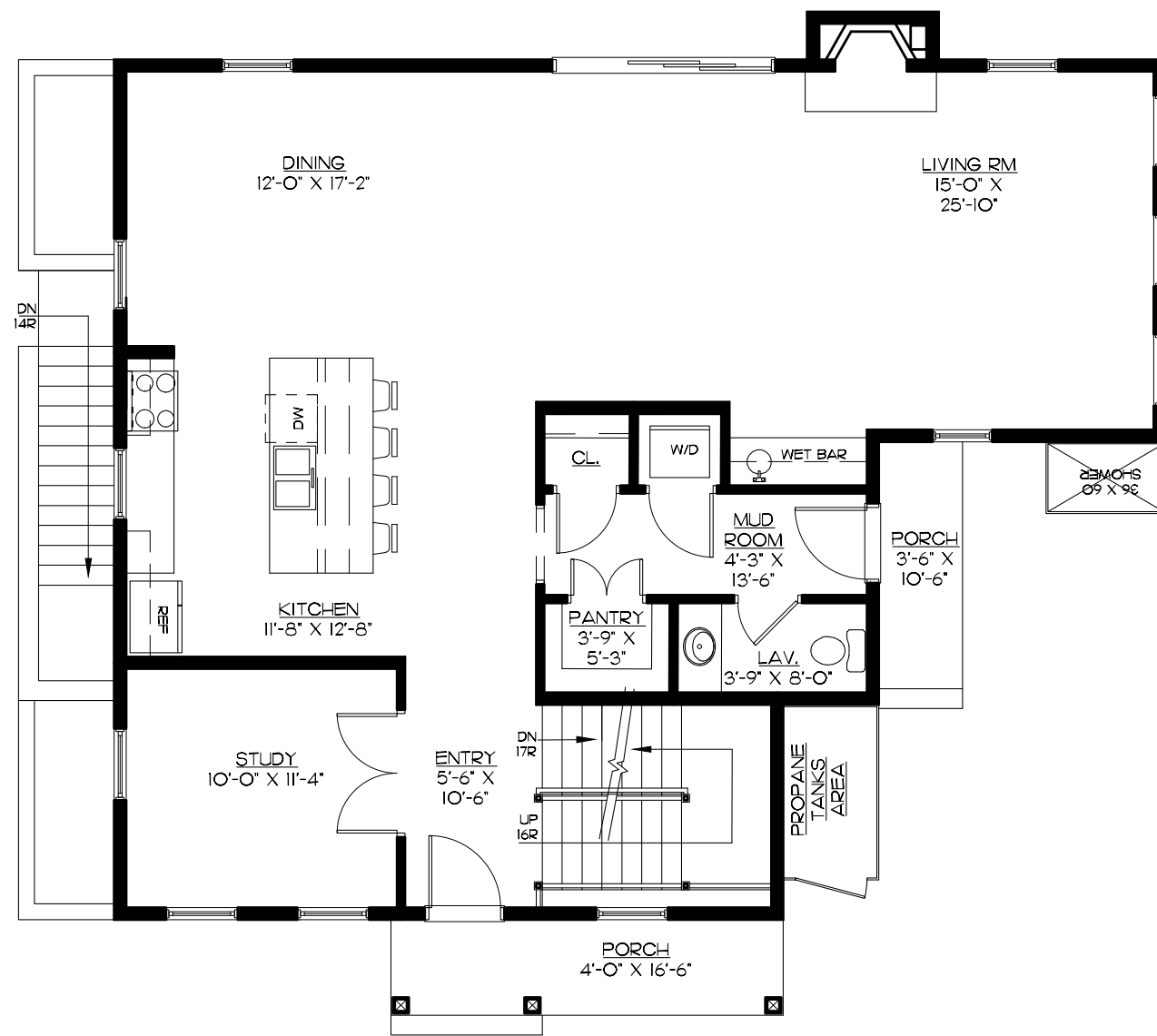
FIRST FLOOR | 1,309 SF
