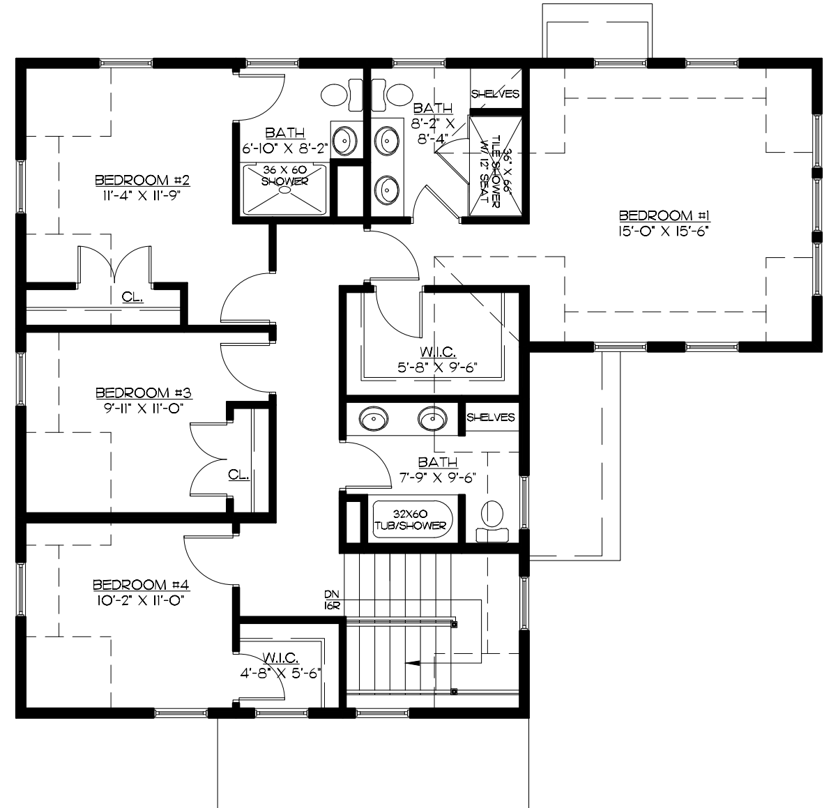
SECOND FLOOR | 1,175 SF
