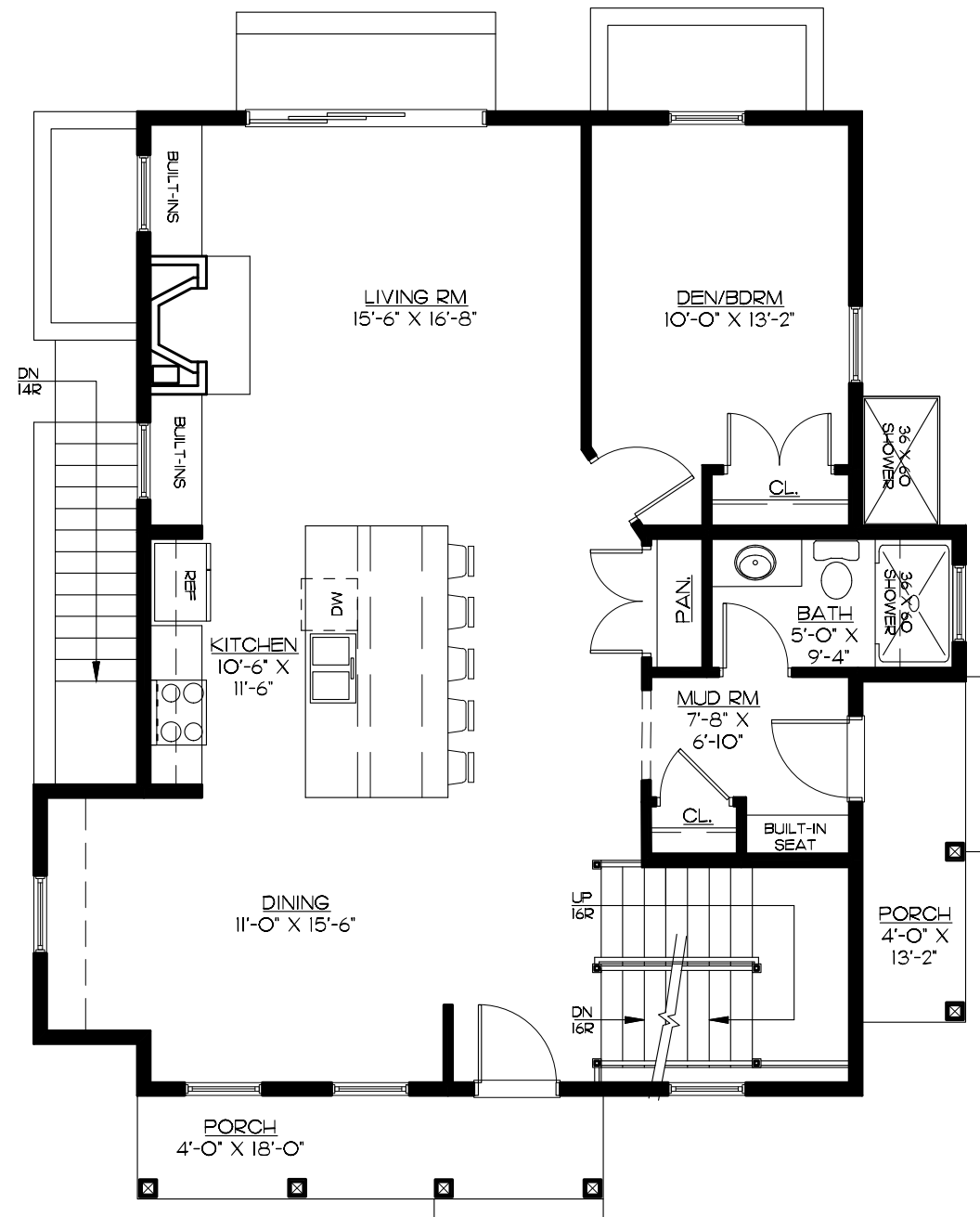
FIRST FLOOR | 1,127 SF
